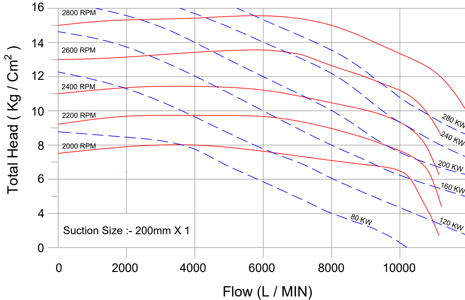
Typical Performance of MFV LP 10000
