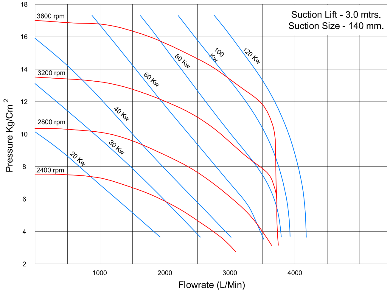
Typical Performance of MFV LP 1030
